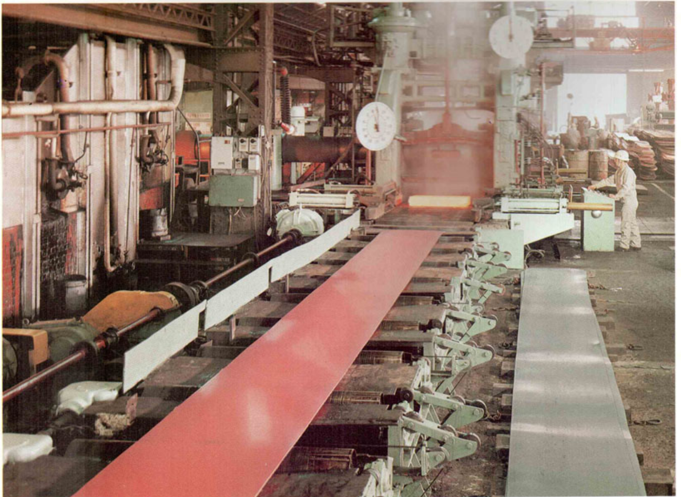
Three high hot breakdown rolling mill.
